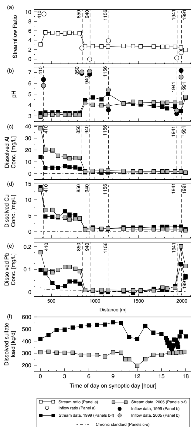
Figure 3. Comparison of 1999 and 2005 data for upper Mineral Creek: (a) ratio of 1999 streamflow to 2005 streamflow, (b) stream and inflow pH, (c–e) dissolved concentrations of Al, Cu, and Pb, (f) time series of sulphate load at 656 m (1999) and 576 m (2005). Vertical lines denote locations of inflow sites
