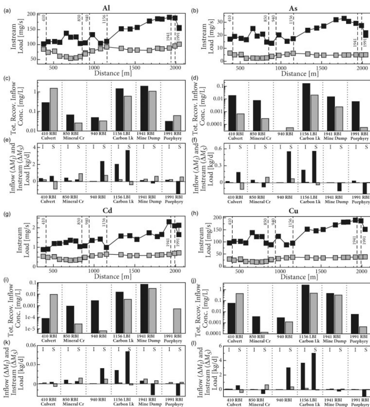
Figure 5. Comparison of 1999 (black symbols) and 2005 (grey symbols) constituent data for upper Mineral Creek: (a, b, g, h, m, n, s, t) spatial profiles of instream load (vertical lines denote locations of inflow sites), (c, d, i, j, o, p, u, v) total-recoverable concentrations at six inflow sites, (e, f, k, l, q, r, w, x) sampled inflow load ( \Delta M_I ) and change in instream load ( \Delta M_S ) for six stream segments with sampled inflows (values of \Delta M_I and \Delta M_S are denoted by I and S, respectively)
