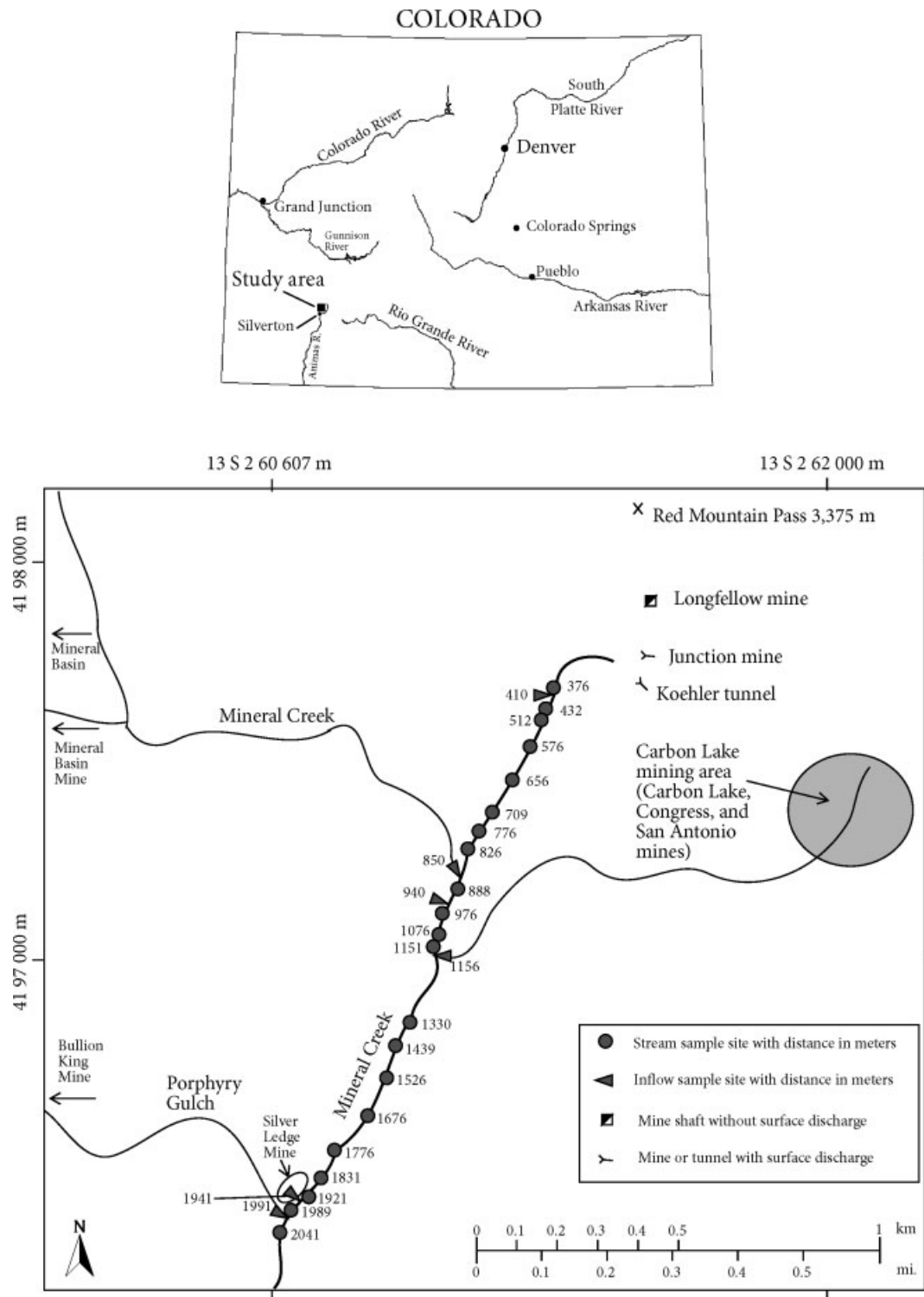
Figure 1. Mineral Creek study reach for September 1999 and August 2005 synoptic sampling
