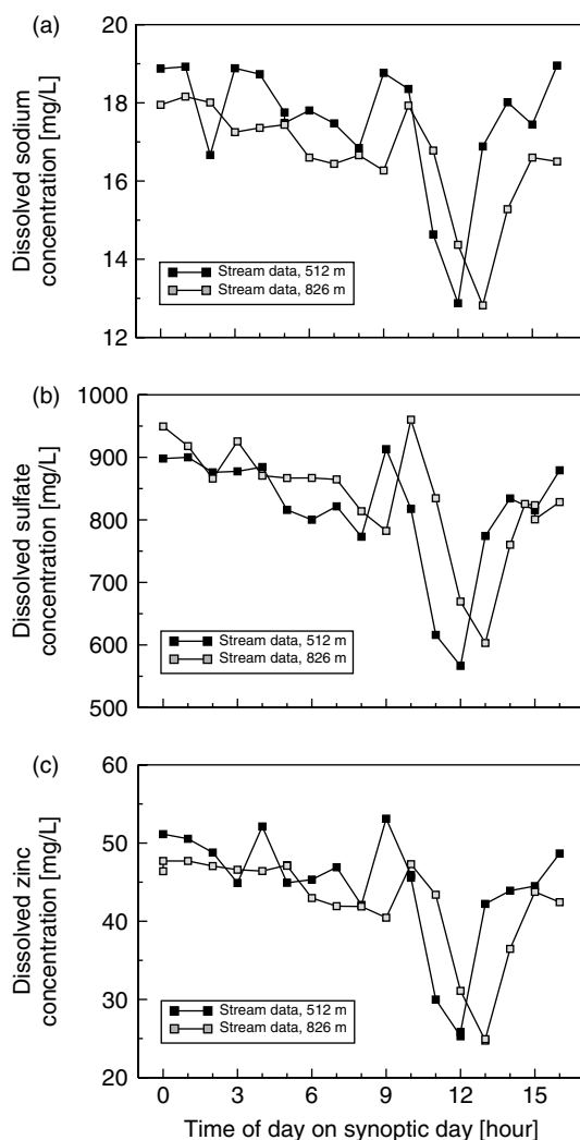
Figure 4. Temporal data at 512 and 826 m on August 22, 2005 for upper Mineral Creek: (a–c) dissolved concentrations of sodium, sulphate, and zinc
