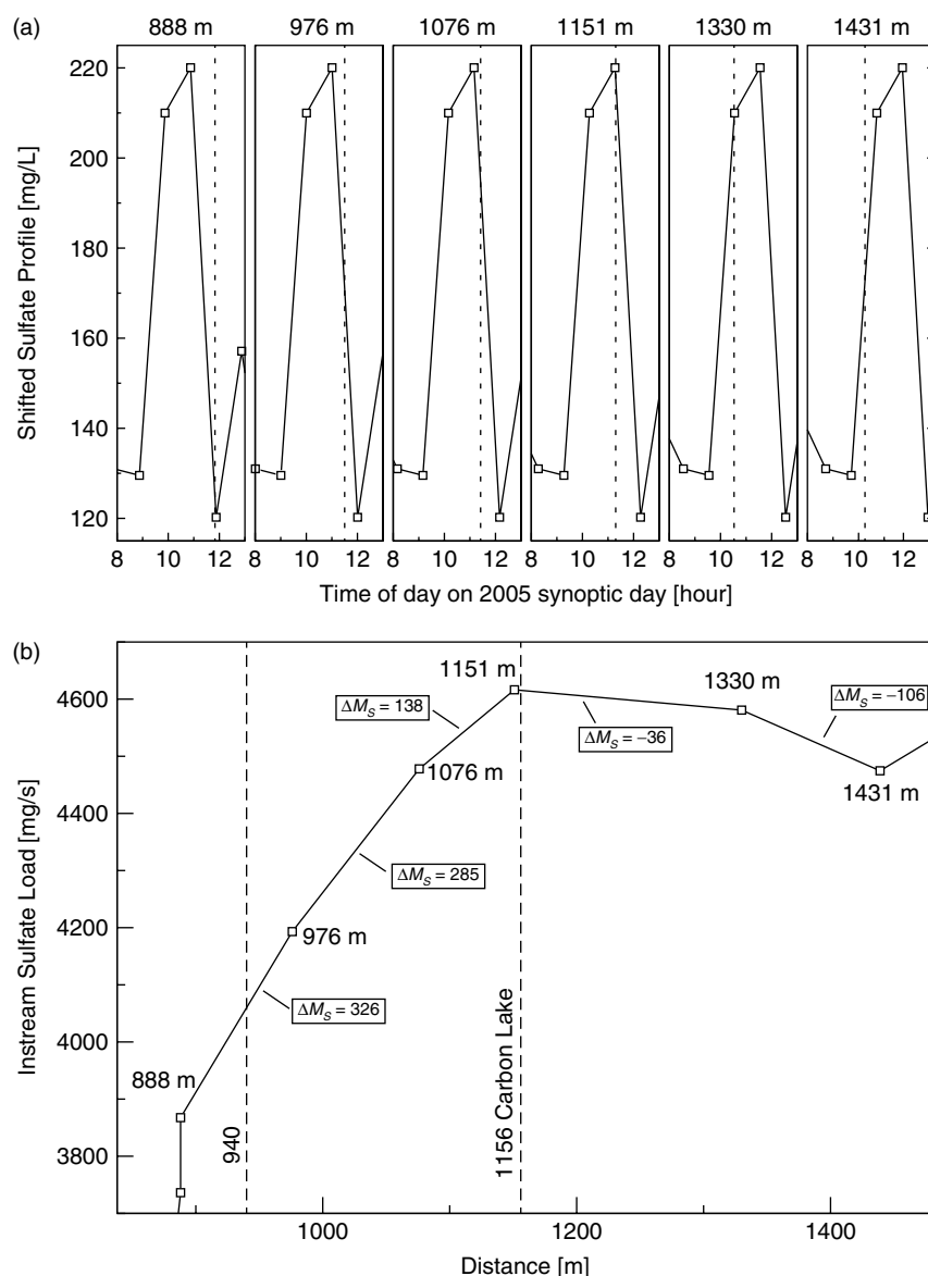
Figure 6. Effect of temporal variation on synoptic sampling: (a) temporal profile of sulphate concentration from 1989 m that has been shifted in time to reflect the sulphate profile that passed the upstream locations. Vertical line represents synoptic sampling time at upstream locations, (b) spatial profile of sulphate load that results from synoptic sampling during period of temporal variability. Increases ( +\Delta M_S ) and decreases ( -\Delta M_S ) in load are an artifact of the temporal variation, rather than actual sources and sinks
