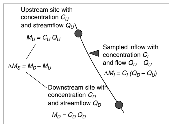
Figure 2. Generic stream segment used to illustrate calculations of mass load
